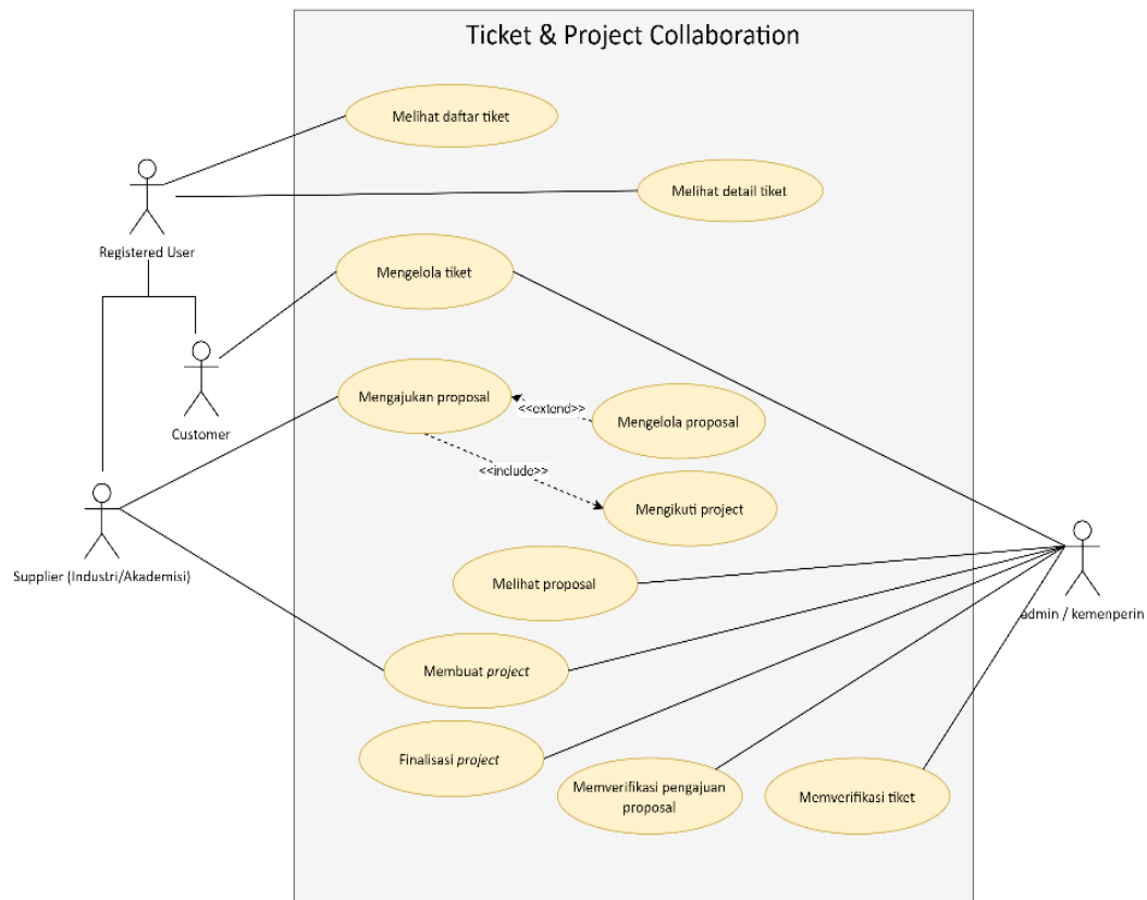
Gambar 3. Usecase Diagram IMC
