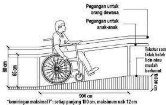
Gambar 1. Ramp Difabel
